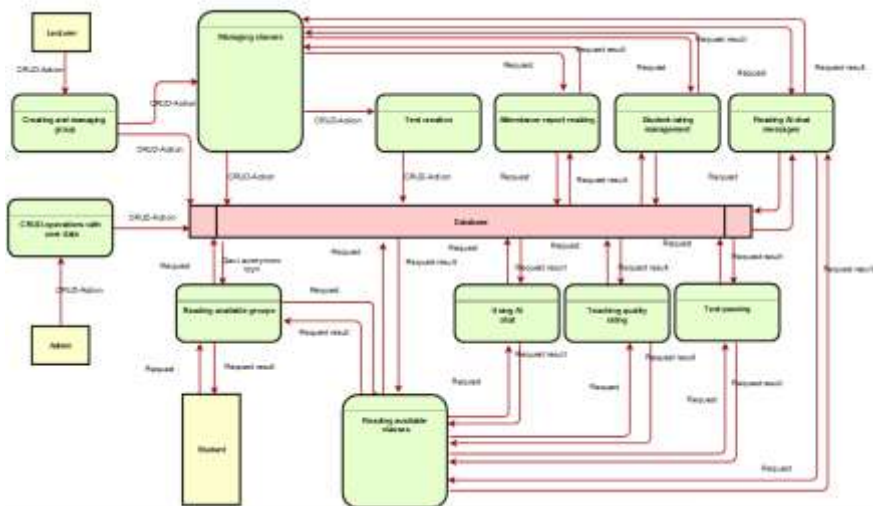
Figure 1: Data flow diagram of the web-application
