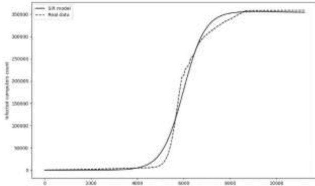
Fig. 1. SIR model of the worm propagation (solid), and the Code Red worm real data (dashed)
